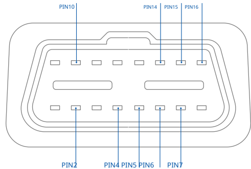
FMB003 Pinout priza OBDII
