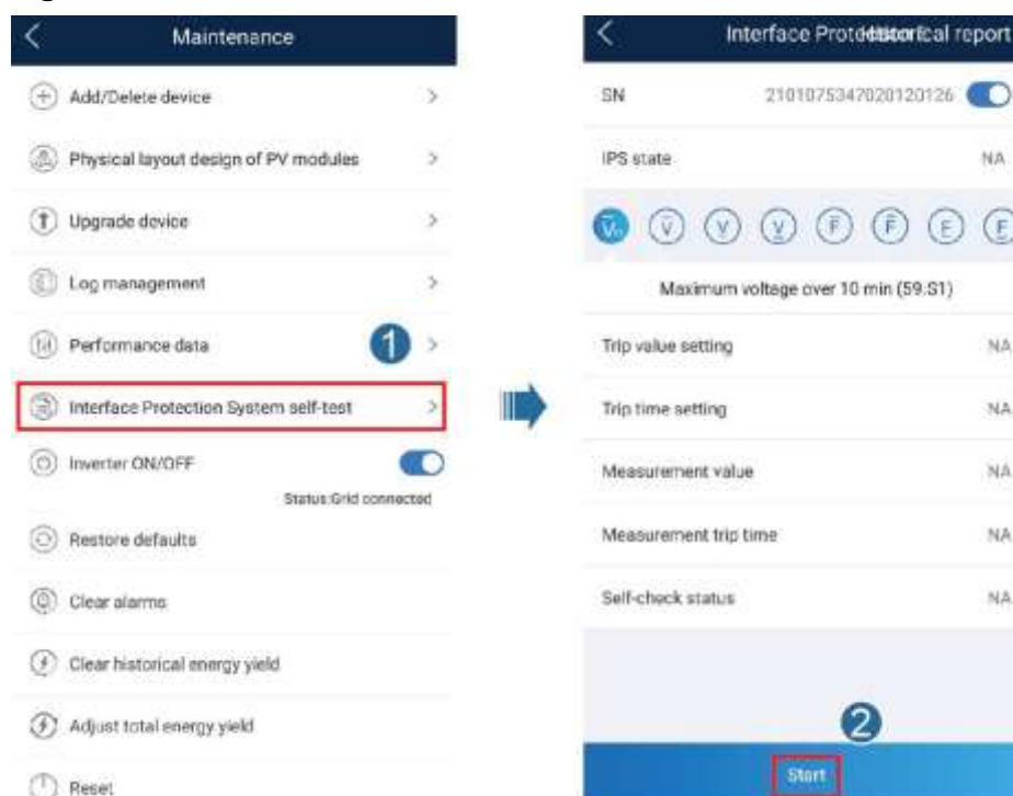
Figura 7-17 Test IPS
