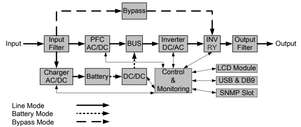
System block diagram
