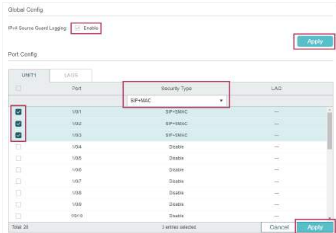
Figure 5-8 IPv4 Source Guard
