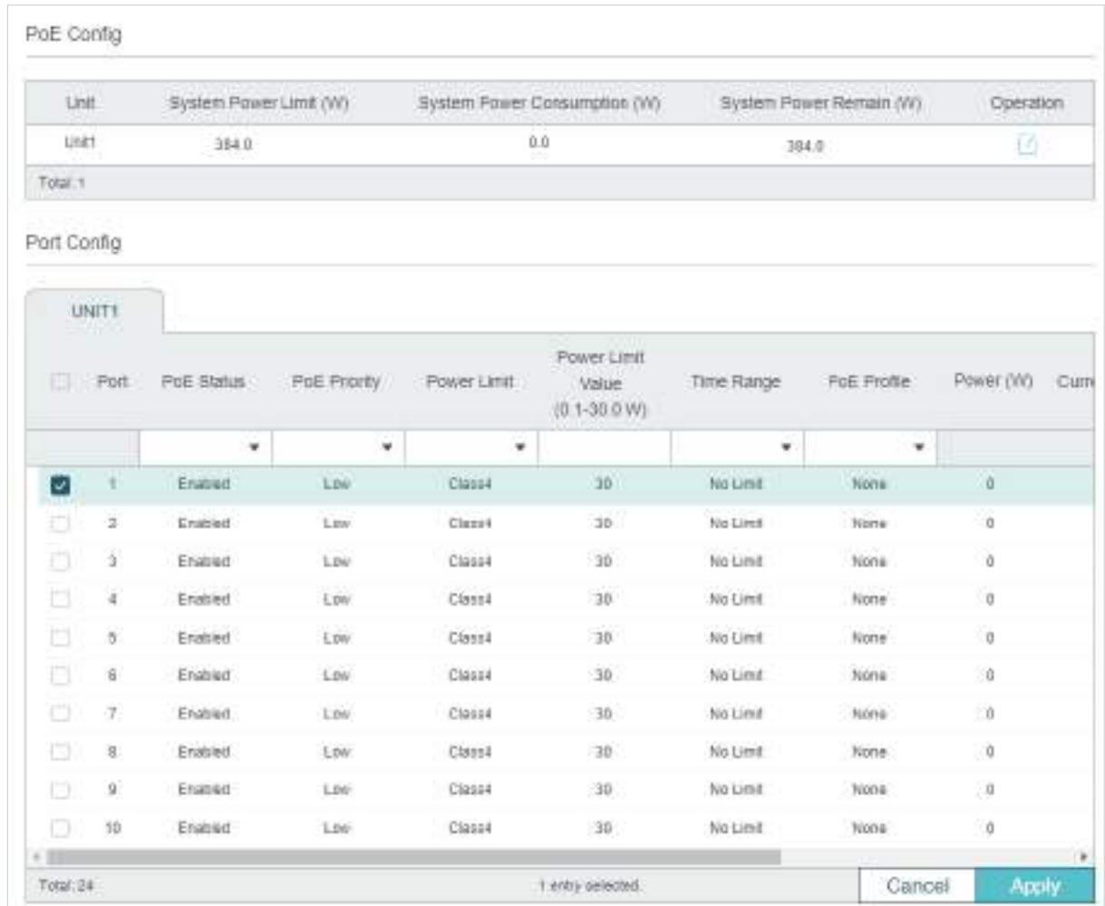
Figure 6-1 Configuring PoE Parameters Manually
