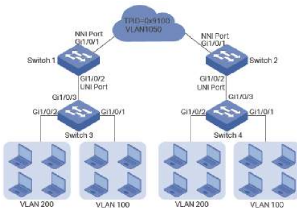
Figure 4-1 Network Topology
