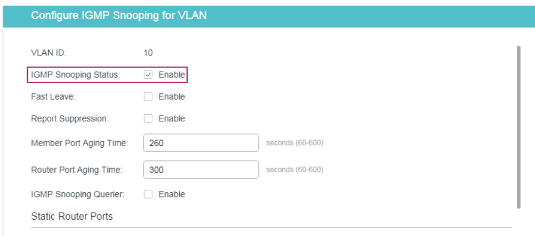
Figure 7-20 Enable IGMP Snooping for VLAN 10
