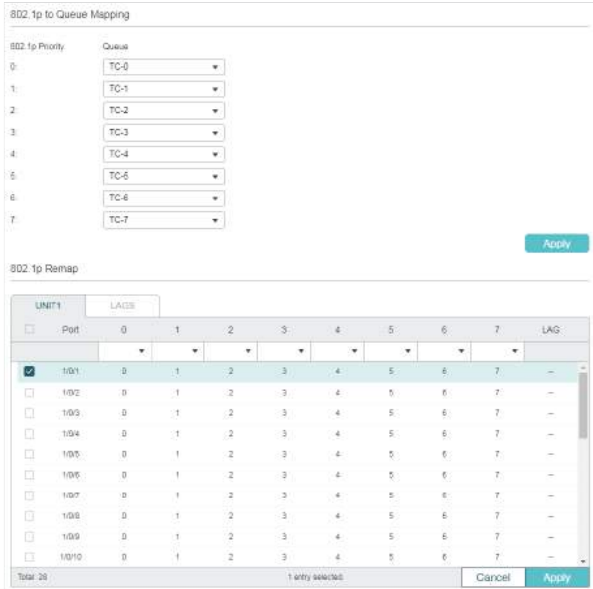
Figure 2-4 Configuring the 802.1p to Queue Mapping and 802.1p Remap
