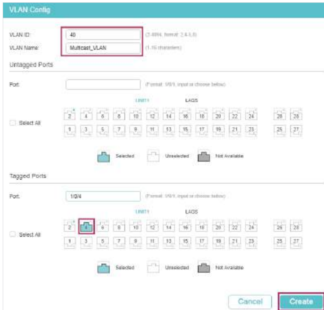
Figure 7-10 Create Multicast VLAN
