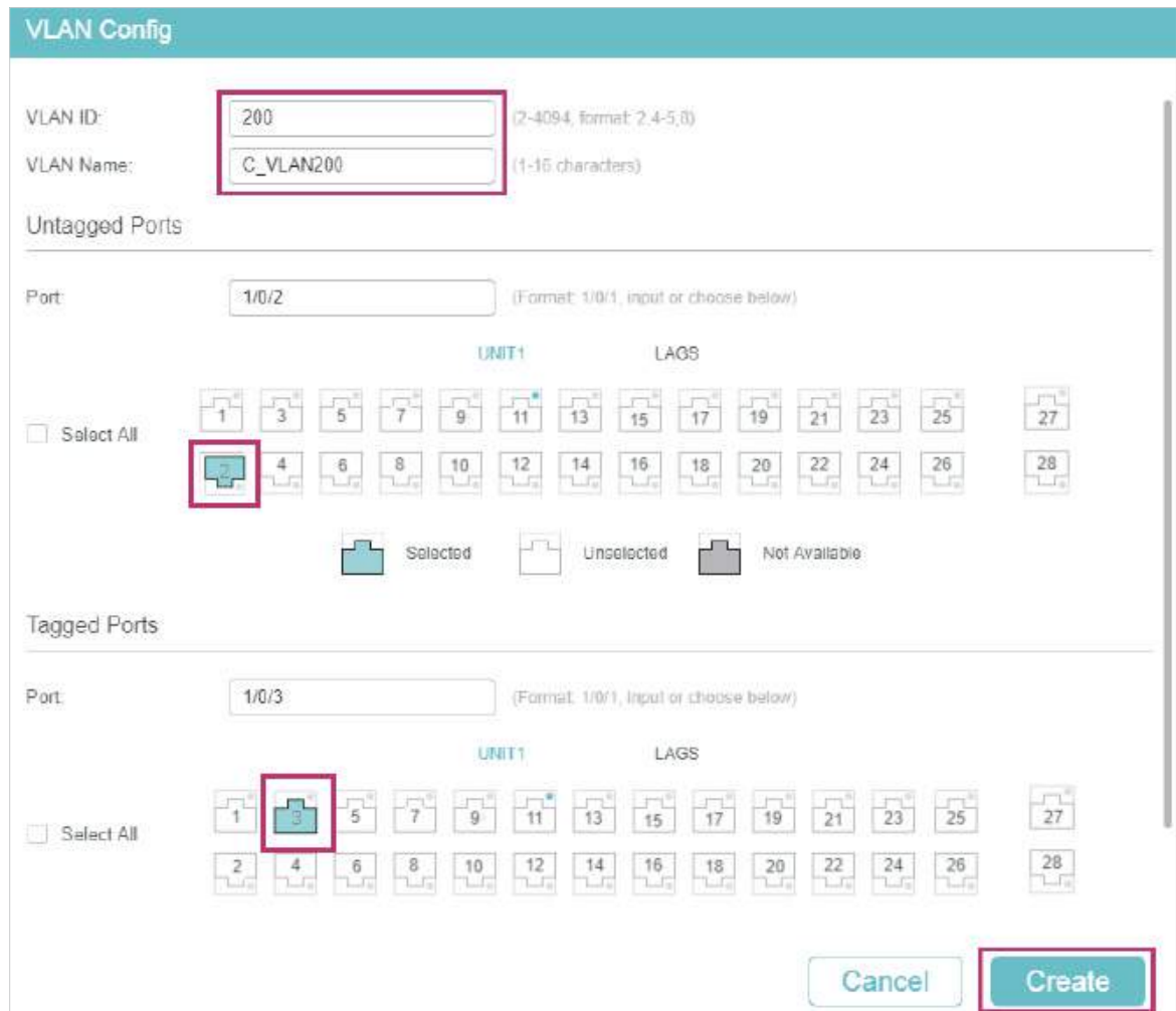
Figure 4-19 Creating VLAN 200
