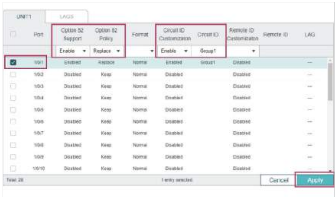
Figure 5-34 Configuring Port 1/0/1
