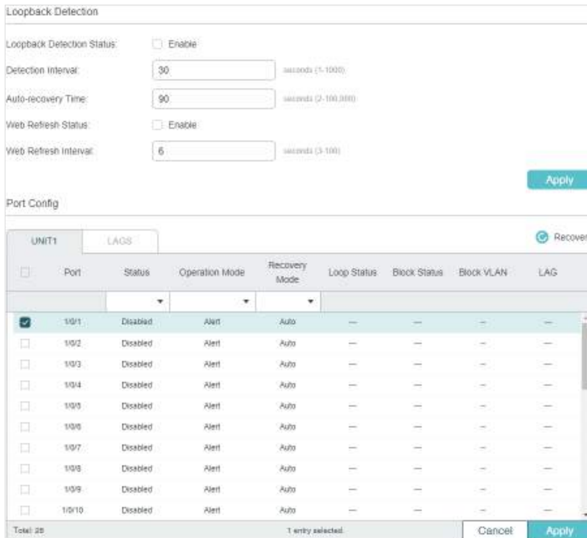
Figure 4-1 Configuring Loopback Detection
