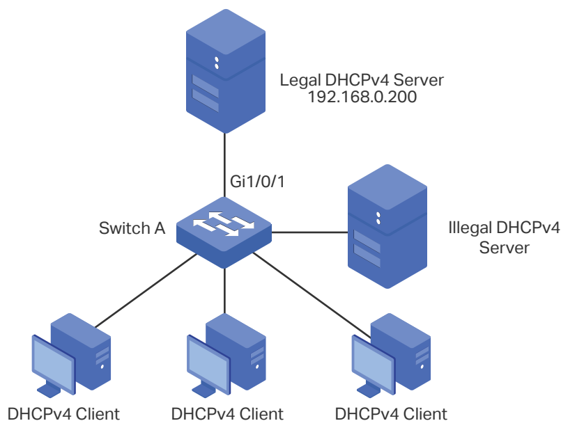
Figure 4-1 Network Topology
