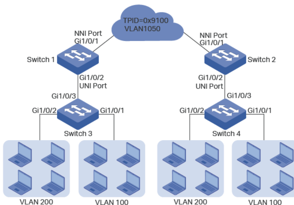
Figure 4-1 Network Topology
