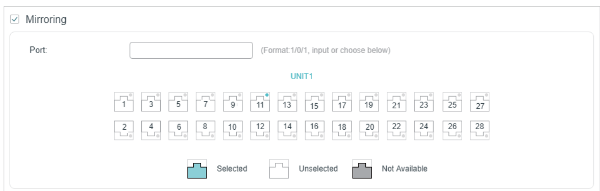
Figure 2-29 Configuring Mirroring
