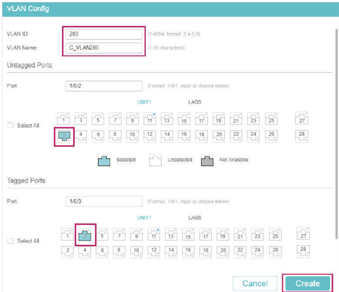
Figure 4-19 Creating VLAN 200
