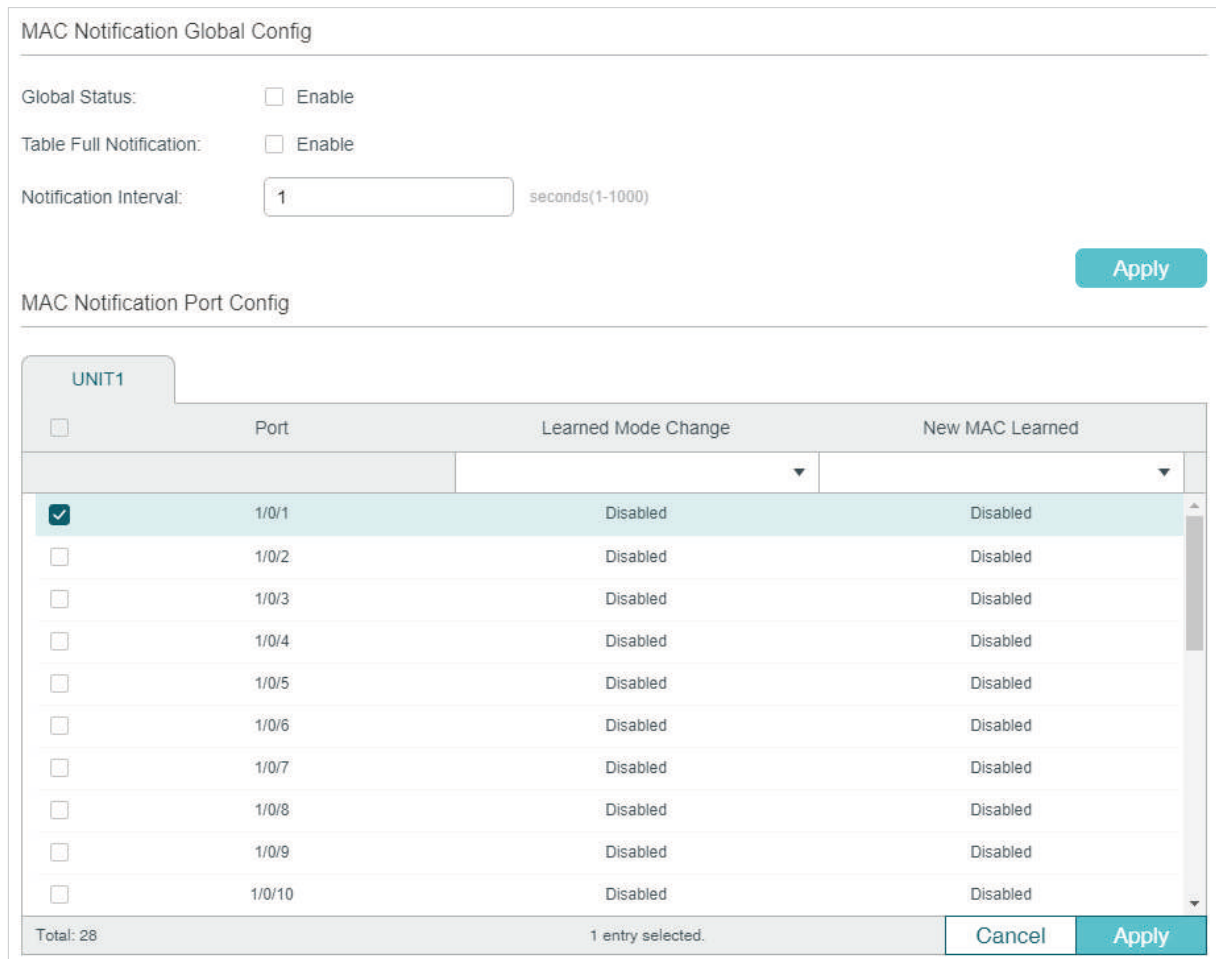
Figure 3-1 Configuring MAC Notification Traps
