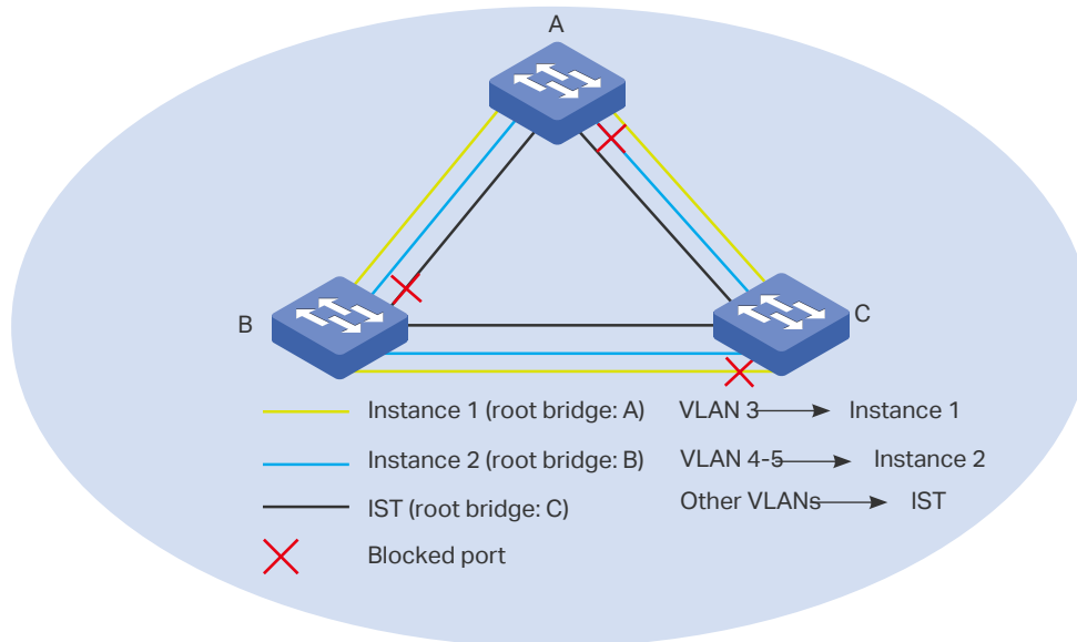
Figure 1-4 MST Region
