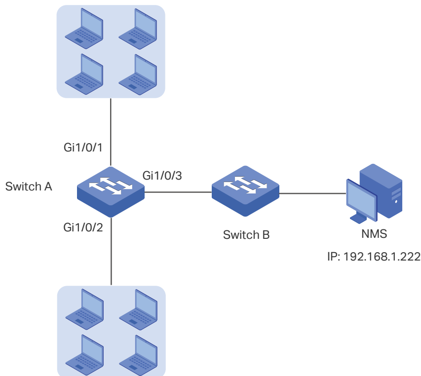
Figure 6-1 Network Topology
