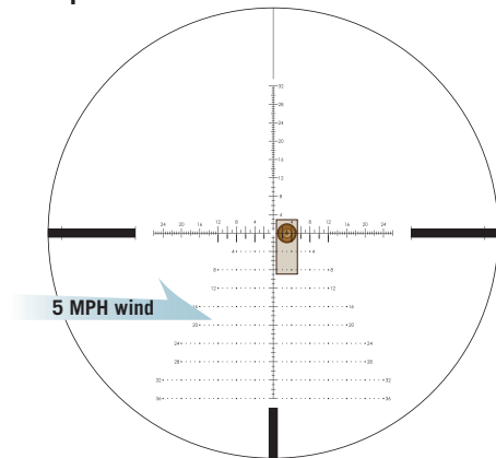
3 MOA reticle windage correction at 700 yds. in 5 MPH crosswind using center crosshair. Elevation adjustment already dialed into the riflescope.
