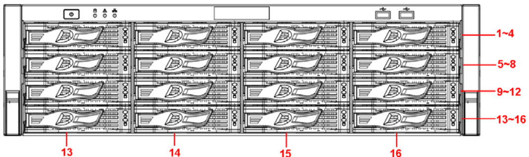
Figura 2-24 Panoul frontal
