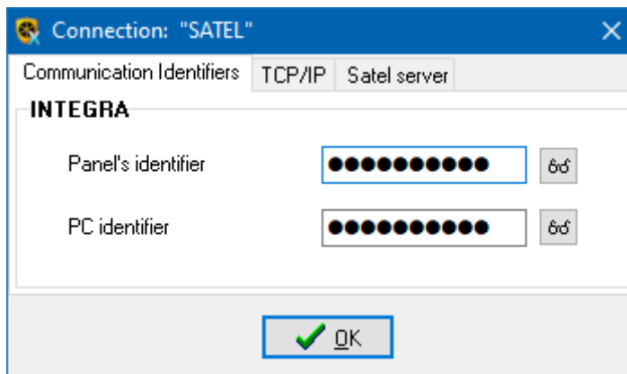
Fig. 16. GUARDX program: "Communication Identifiers" tab in "Connection" window.
