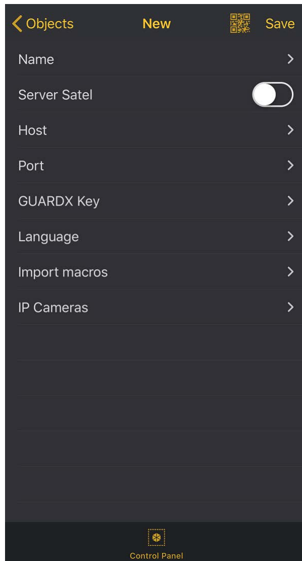
Fig. 22. INTEGRA CONTROL application (iOS system): the screen for adding a control panel.
