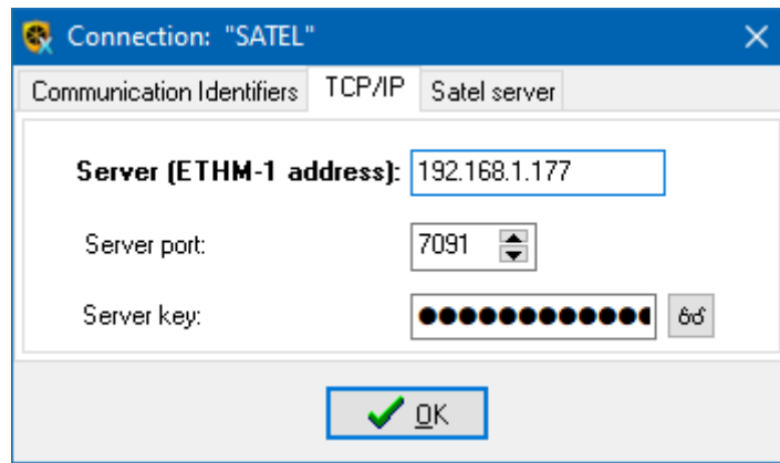
Fig. 17. GUARDX program: “TCP/IP” tab in “Connection” window.
