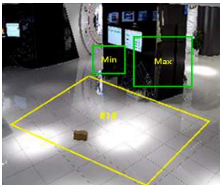
Figure 6-8 Set Rule
