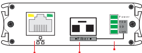
Port Ethernet Port SFP LED Status
