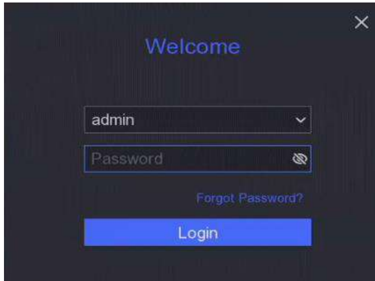
Figure 1-4 Login Interface
