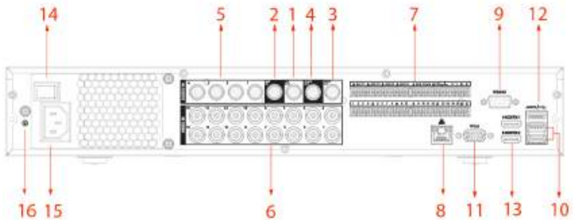
Figure 3-20 Rear panel (3)
