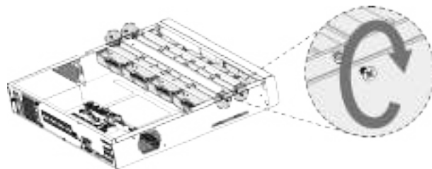
Figure 2-21 Fasten screws
