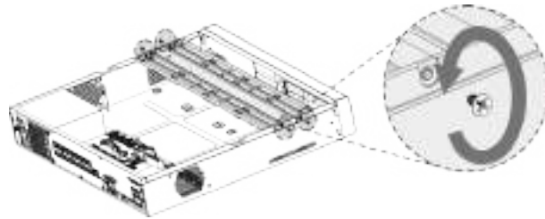
Figure 2-18 Remove bracket
