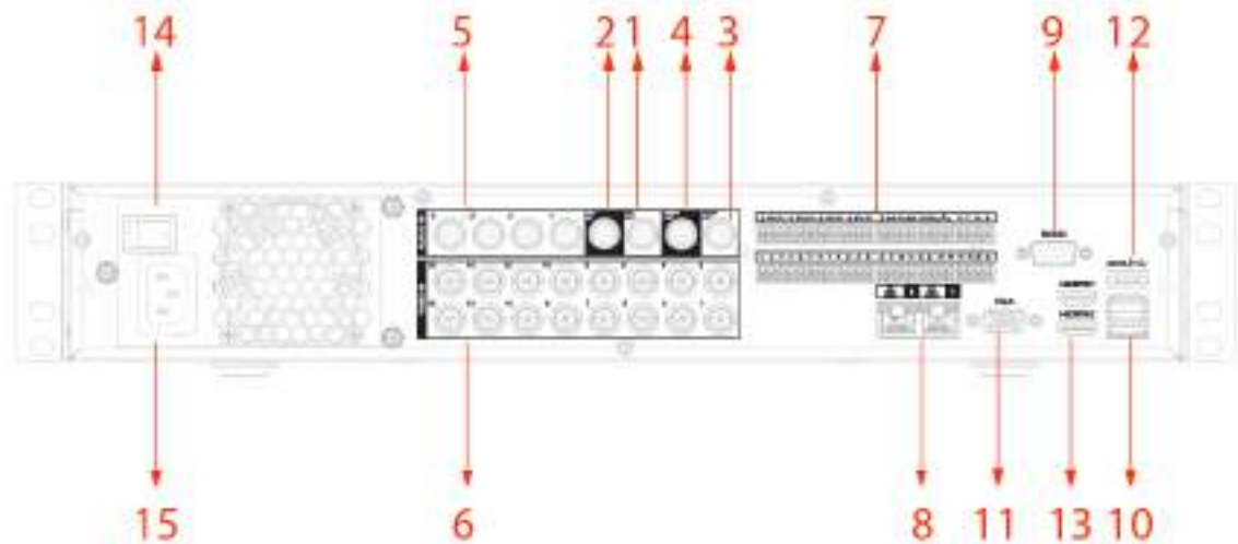
Figure 3-20 Rear panel (3)
