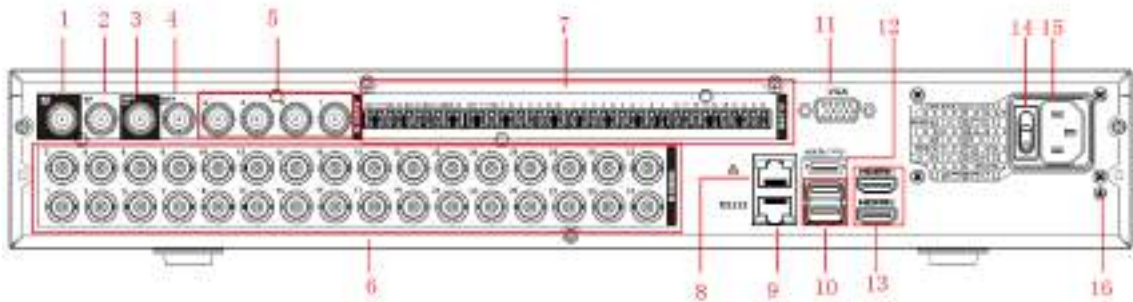
Figure 3-19 Rear panel (2)
