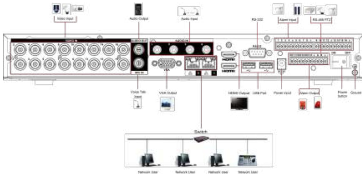
Figure 4-1 Connection diagram
