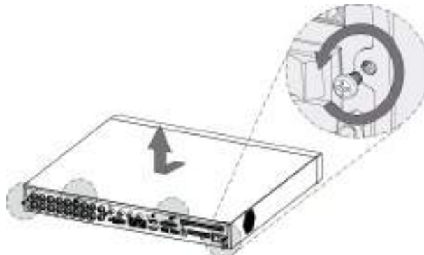
Figure 2-1 Remove screws
