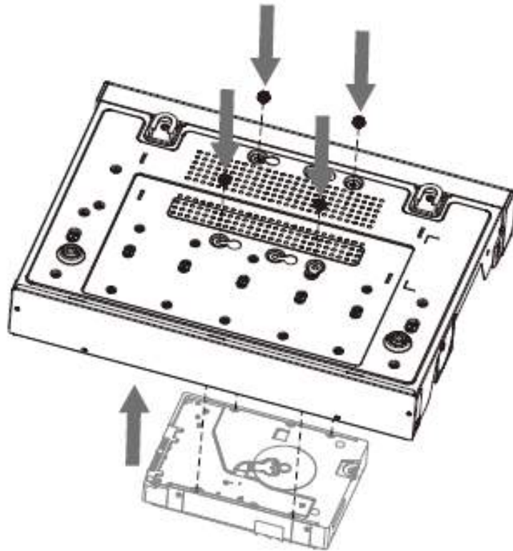
Figure 2-26 Fasten screws
