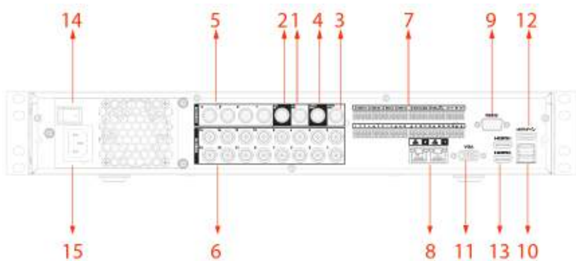
Figure 3-20 Rear panel (3)
