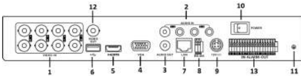
Figure 1-8 Rear Panel of DS-7200HUHI-K and iDS-7200HUHI-K/4S
