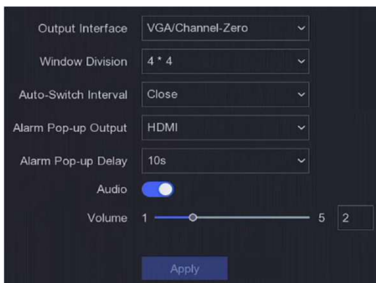
Figura 6-2 Live View-General
