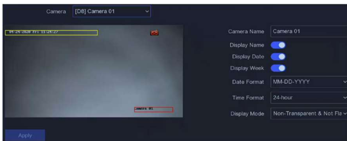
Figura 5-11 OSD
