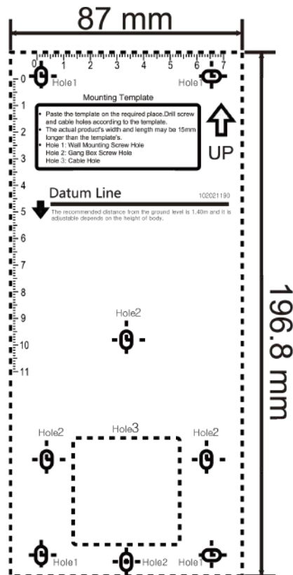
Figure 3-4 Mounting Template
