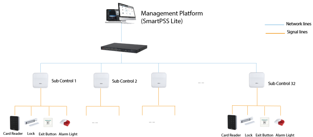
Figure 3-1 Networking Diagram
