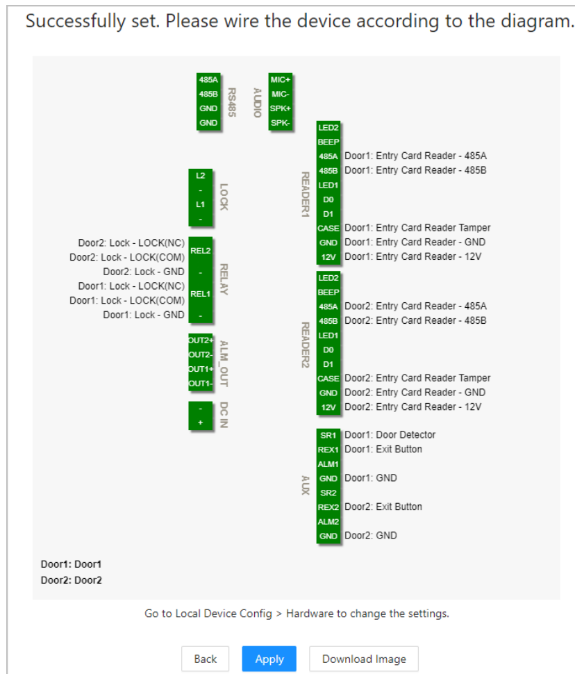
Figure 2-8 Wiring diagram
