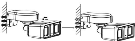
Figure 2-11 Lock Cover to Body
