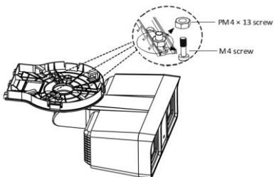
Figure 2-9 Secure Camera to Wall Mount Cover
