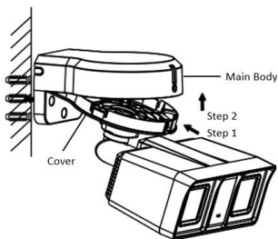
Figure 2-10 Secure Cover to Body
