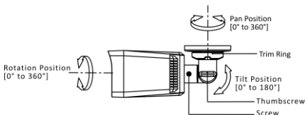
Figure 2-2 3-Axis Adjustment
