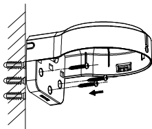
Figure 2-8 Secure Main Body to Wall
