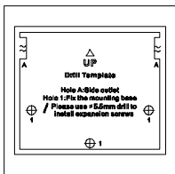
Figure 2-7 Drill Template for Wall Mount
