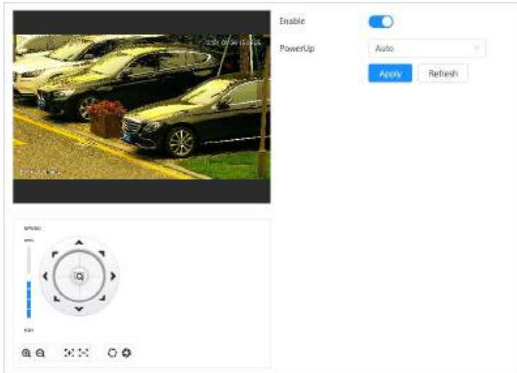
Figure 4-53 Power up
