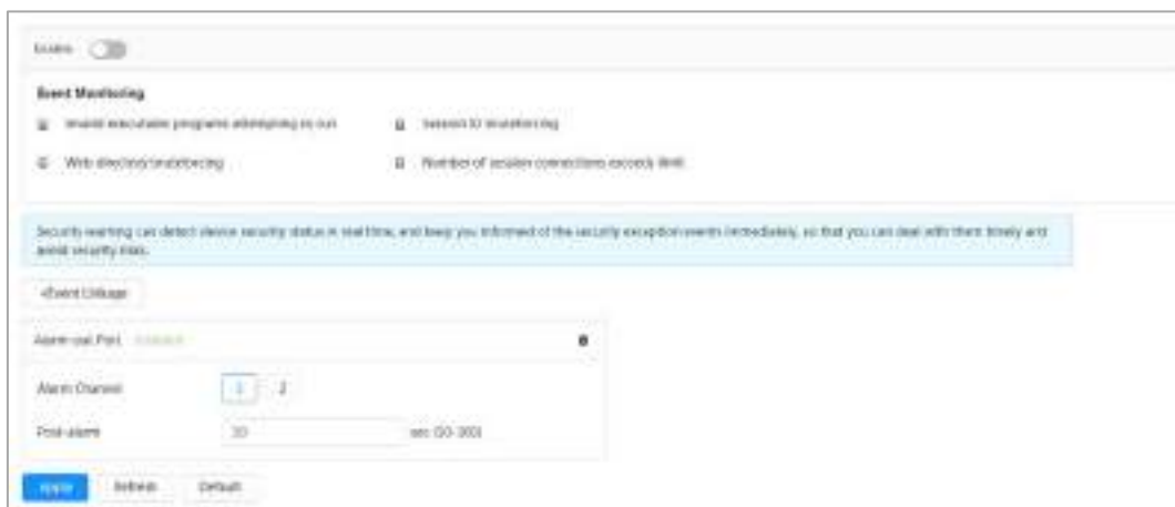
Figure 9-15 Security warning
