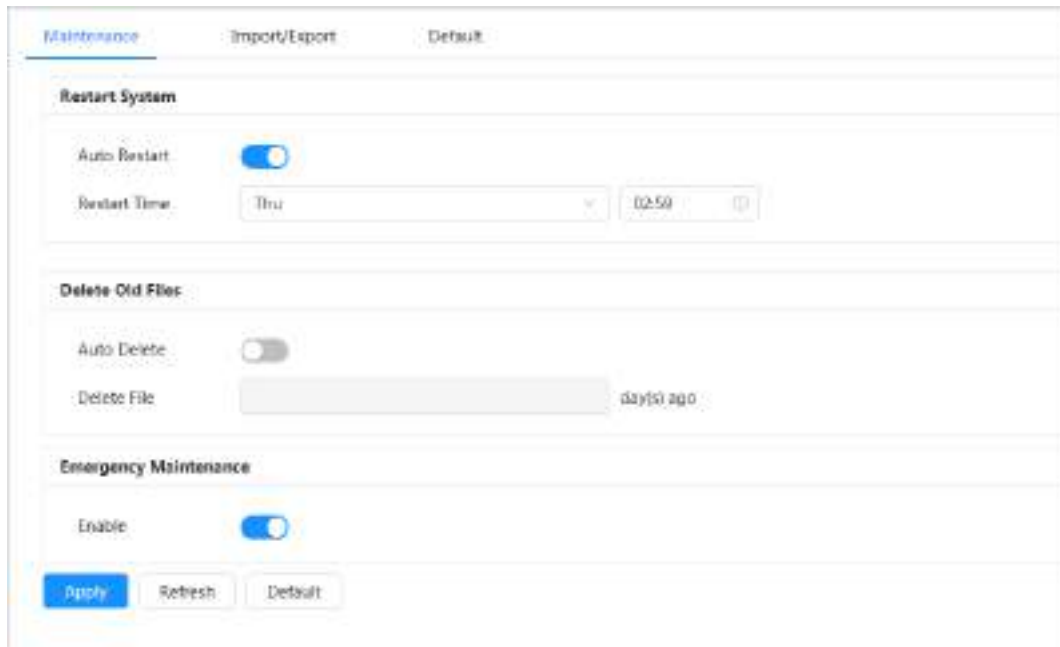
Figure 4-89 Maintenance
