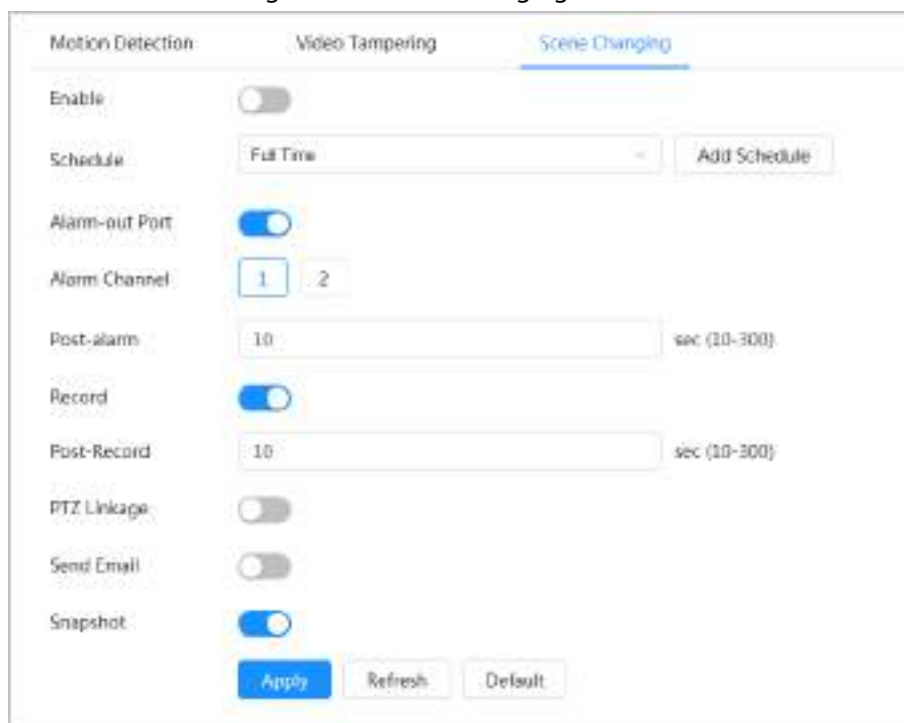
Figure 4-73 Scene changing
