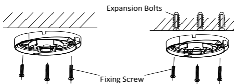
Figure 2-12 Fix the Mounting Base to the Ceiling
