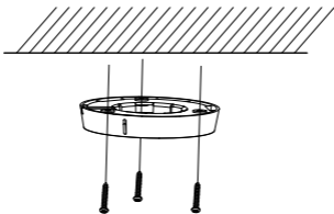
Figure 2-4 Fix the Mounting Base
