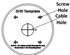
Figure 2-10 Drill Template
